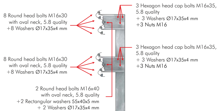
Detail of joint between barriers
