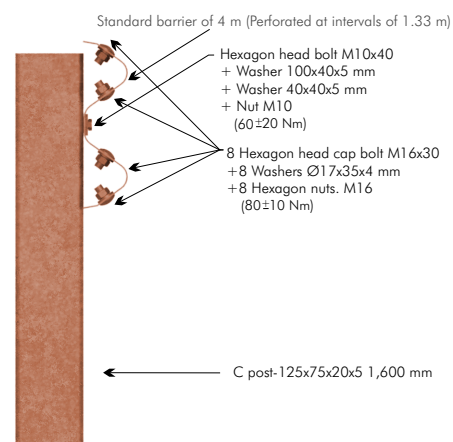
Detail of joint between barriers
