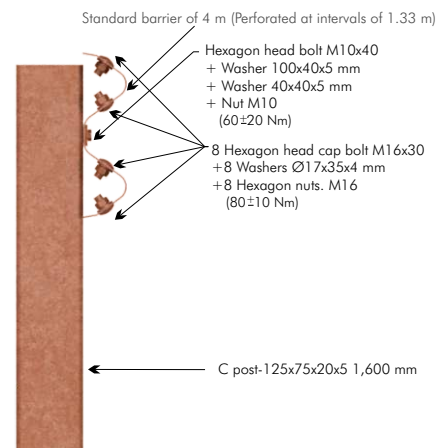
Detail of joint between barriers
